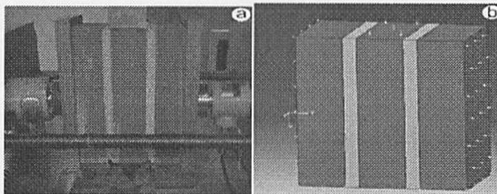
Figure 3 .Supports and loads condition of the specimen in experimental tests (a) and numerical modeling (b).
