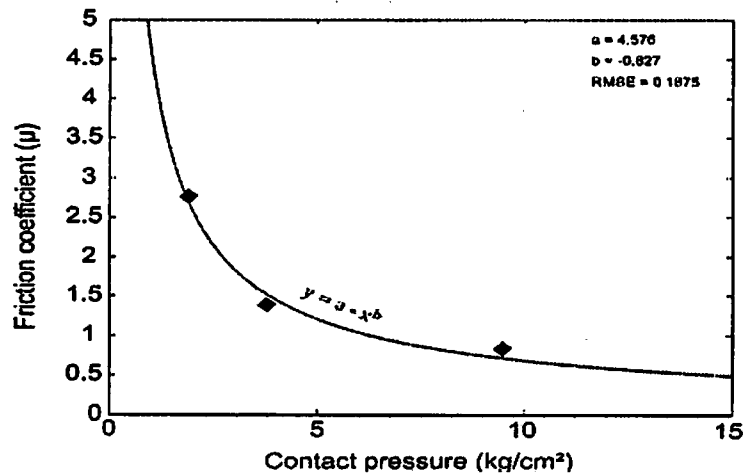
Figure 8. Contact pressure and friction coefficient relationship.
