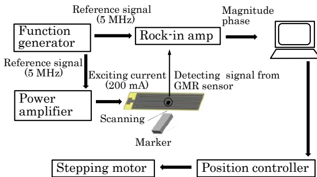
Fig. 9 Measurement system.
