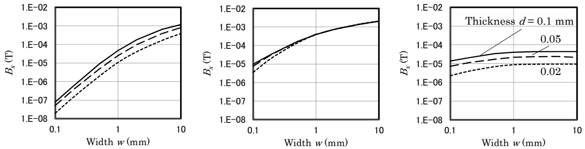
(a) Conductive ink ( \mu^* = 1, \sigma = 3 \times 10^5 \text{ S/m} ) (b) Metal ( \mu^* = 1, \sigma = 6 \times 10^7 \text{ S/m} ) (c) Magnetic ink ( \mu^* = 10, \sigma = 0 )
