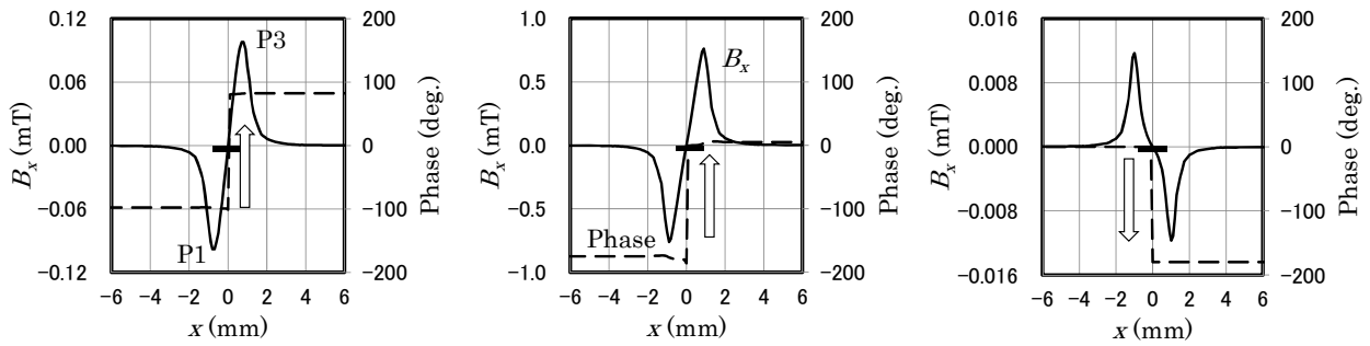
(a) Conductive ink ( \mu^* = 1, \sigma = 3 \times 10^5 \text{ S/m} ) (b) Metal ( \mu^* = 1, \sigma = 6 \times 10^7 \text{ S/m} ) (c) Magnetic ink ( \mu^* = 10, \sigma = 0 )
