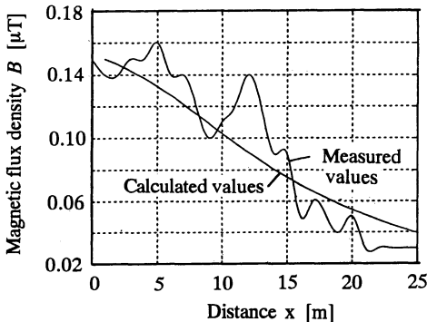
Fig. 5 Magnetic field distribution near a power transmission line.
