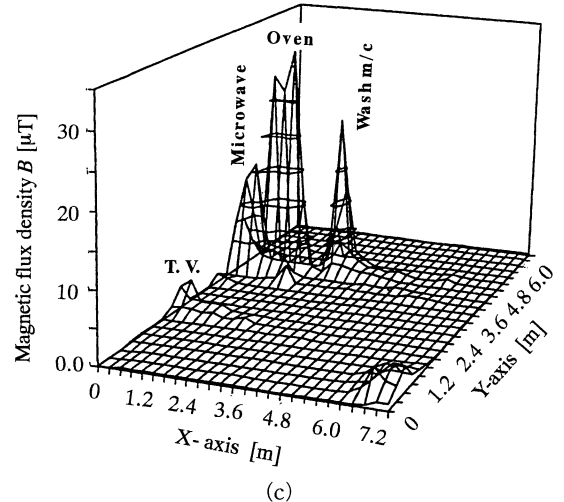
Fig. 4 Spot measurements in a household. (a) The floor arrangement of a household. (b) Magnetic field distribution with electric equipment switched off. (c) Magnetic field distribution with switched on.
