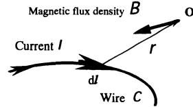
Fig. 2 BIOT-SAVART equation.
