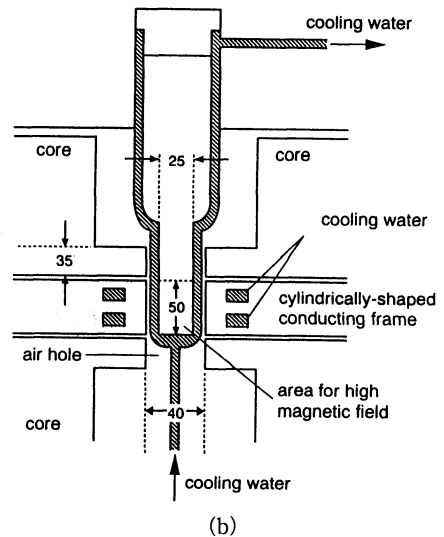
Fig. 6 AC high magnetic field generator.
