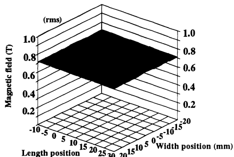
Fig. 9 Magnetic field distribution.
