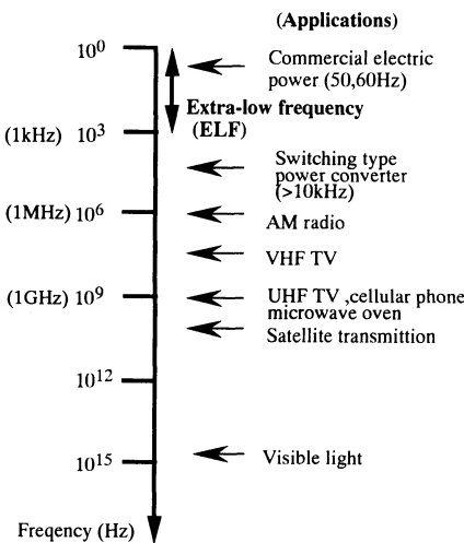
Fig. 1 Electromagnetic spectrum.
