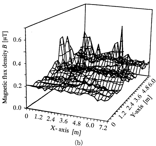
Fig. 4 Spot measurements in a household. (a) The floor arrangement of a household. (b) Magnetic field distribution with electric equipment switched off. (c) Magnetic field distribution with switched on.
