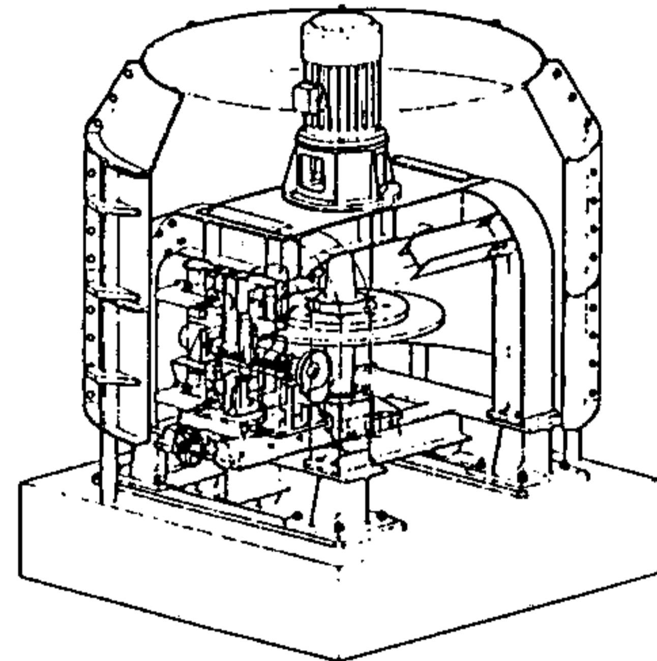
Fig.6 Experimental apparatus
