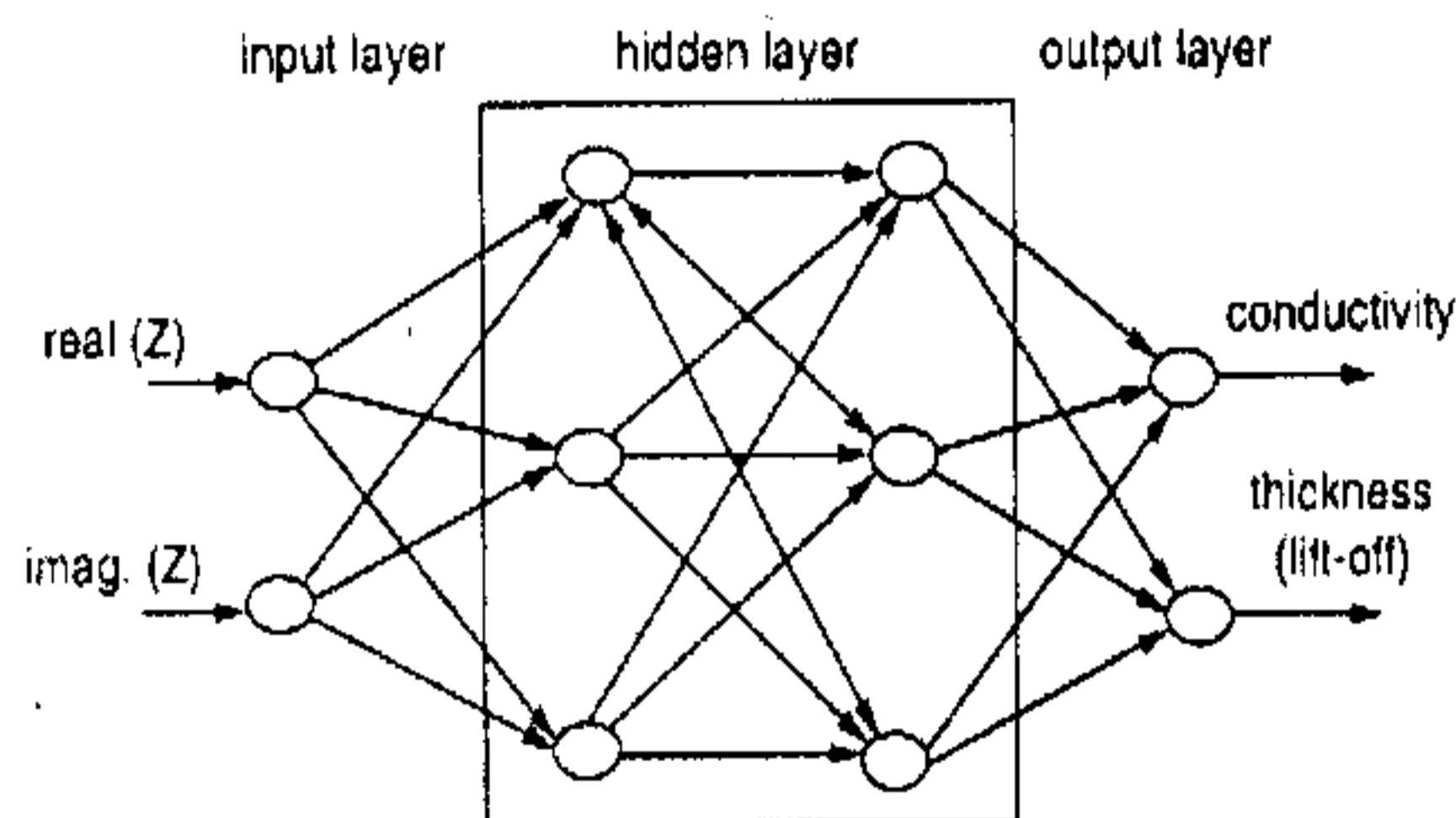
Fig. 9. Schematic representation of neural network model.
