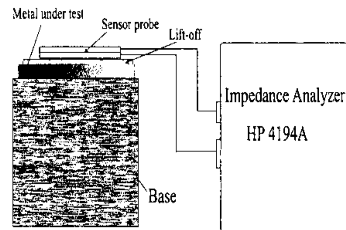
Fig. 7. Experimental setup.
