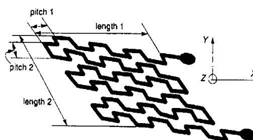
Fig. 2. Configuration of mesh-type magnetic sensor.
