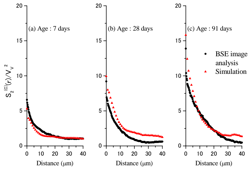
Figure 8 Normalized two-point correlation functions for unhydrated cement particles : (a) 7days (b) 28days (c) 91days
