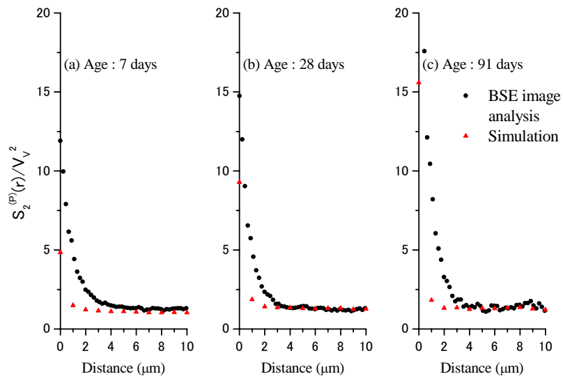
Figure 11 Normalized two-point correlation functions for capillary pores: (a) 7 days (b) 28 days (c) 91 days
