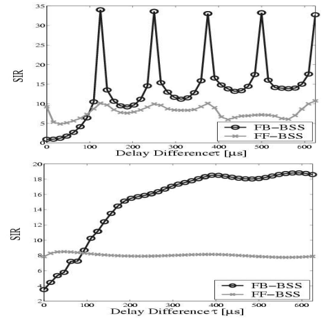
Fig. 5. SIR with respect to \tau for (Upper) white signal sources with instantaneous and delay mixture and (Lower) speech signal sources with room acoustic mixture.
